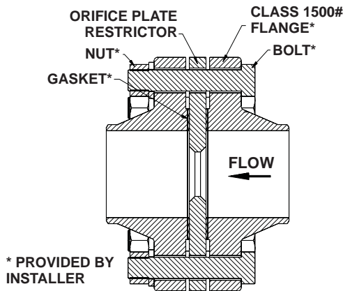
Figure 12. Flow Restrictor
